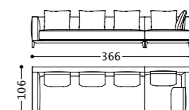
01DYL6 (1DYL230SX + 1DYL280DX) 02DYL6 (2DYL230SX + 2DYL280DX)
