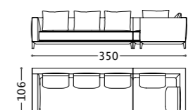
01DYL11 (1DYL230SX + 1DYL260DX) 02DYL11 (2DYL230SX + 2DYL260DX)
