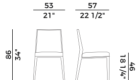
765/II sedia \ chair
