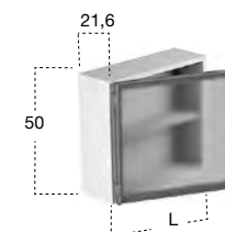
Art. KE1436 / KE1445 / KE1454 Versione sx / Left version
