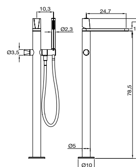
art. ND903LU art. ND903GR
