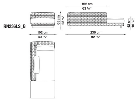
RN236LS_B
